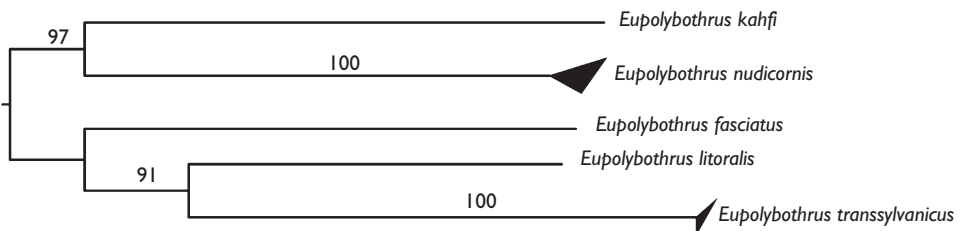
Figure 5. Neighbor joining tree (K2P) of 5 species of Eupolybothrus based on the COI 5' 'barcoding fragment'. Bootstrap support values are shown on the branches. The upper and lower sides of the triangle represent respectively the maximum and minimum of genetic distances within the species.
